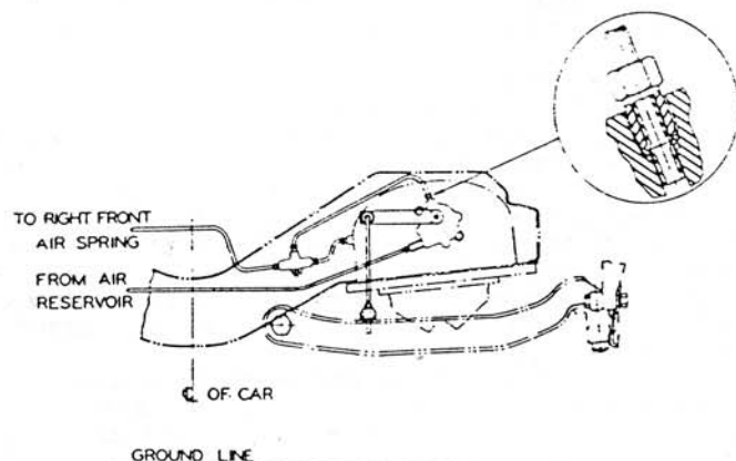
Fig. 17—Leveling valve
