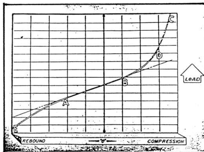
Fig. 1—Ideal load-deflection curve
