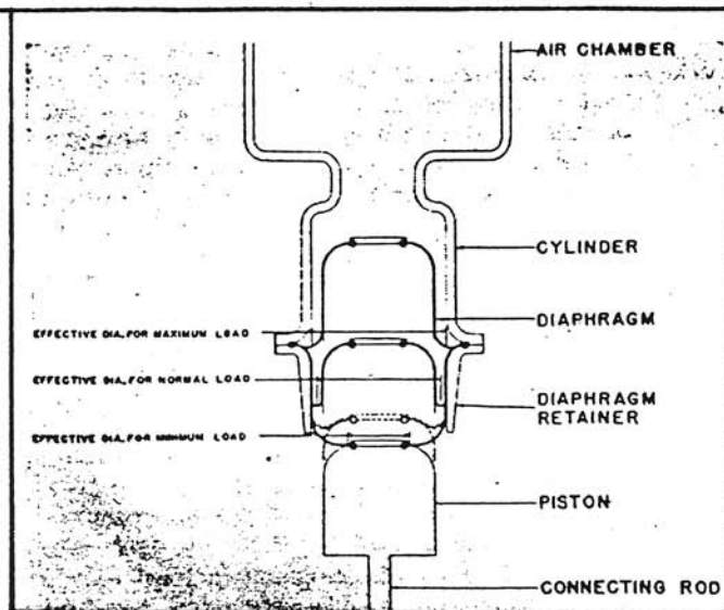
Fig. 3—Variable-area piston
