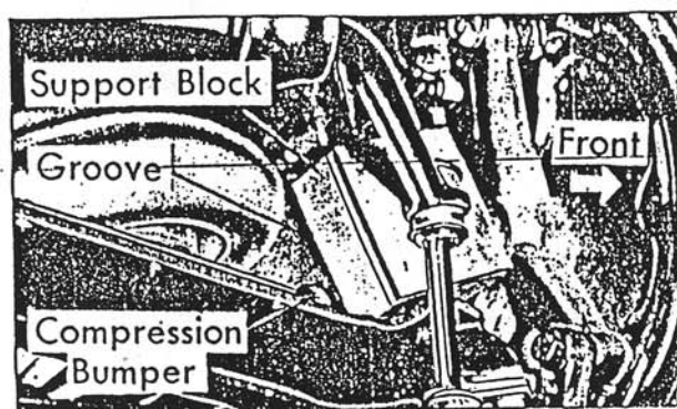
Fig. 4-8 Front Towing Block Installed
