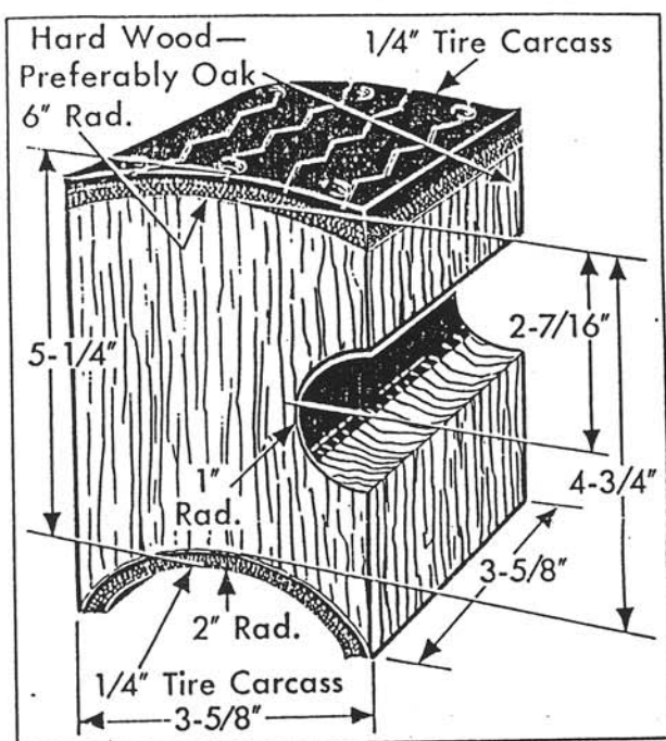
Fig. 4-6 Towing Block Specifications
